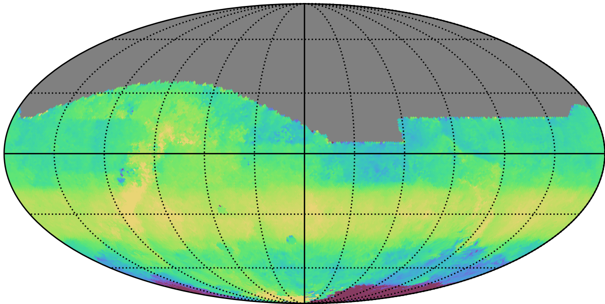
too_elab_r32_d2_gz_v3.4_10yrs All sky z band: Median HA
