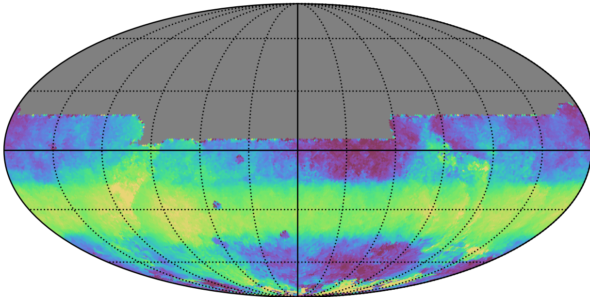
too_elab_r32_d2_gz_v3.4_10yrs All sky y band: Median HA
