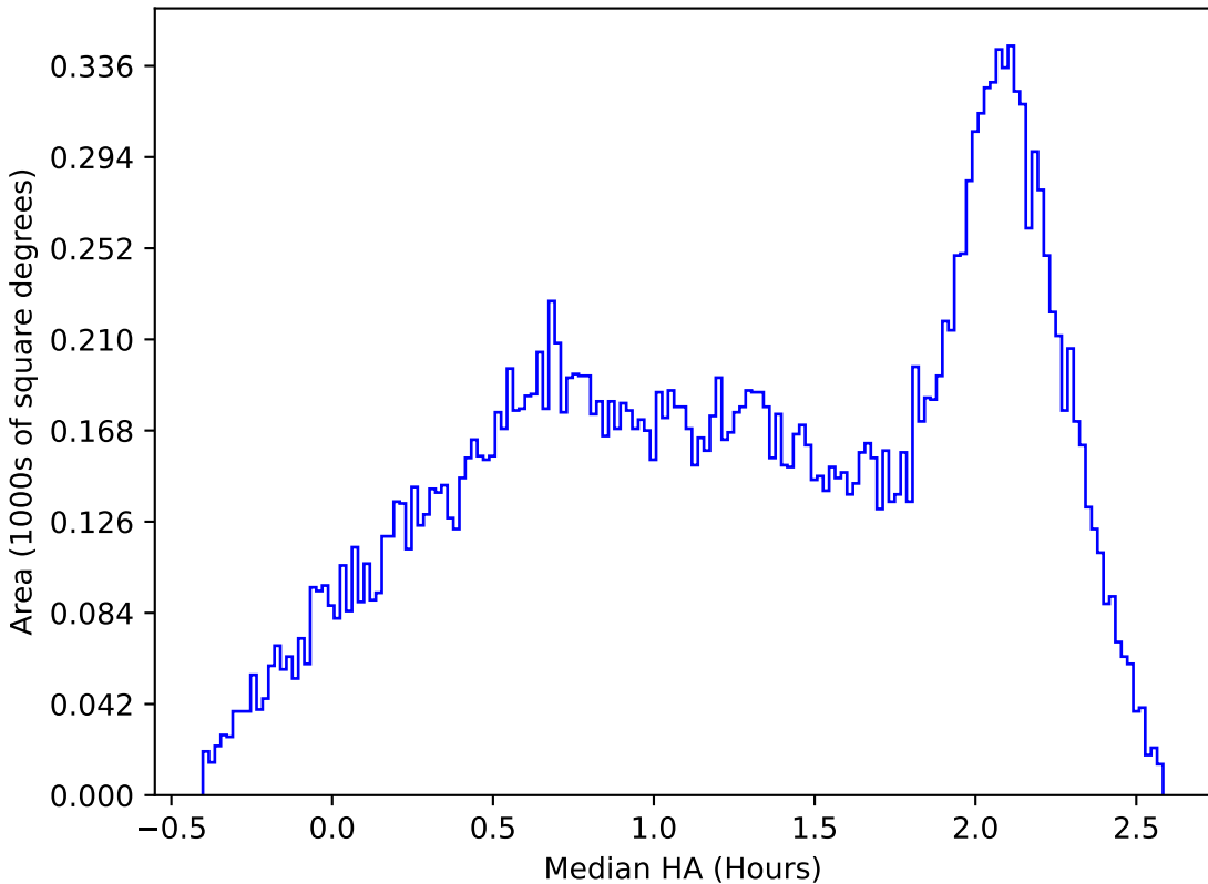
too_elab_r32_d2_gz_v3.4_10yrs All sky y band: Median HA
