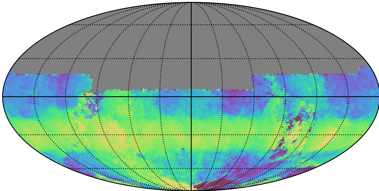
too_elab_r32_d2_gz_v3.4_10yrs All sky u band: Median HA
