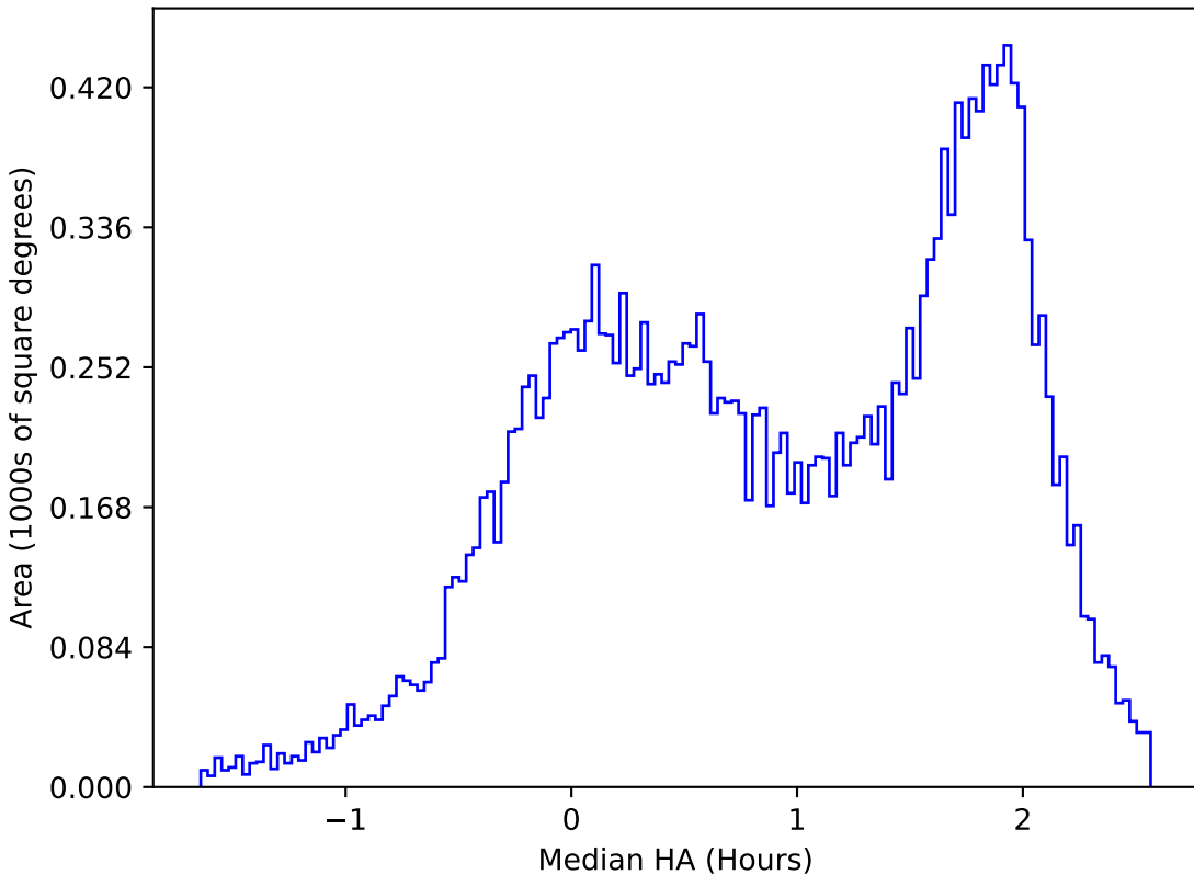
too_elab_r32_d2_gz_v3.4_10yrs All sky u band: Median HA
