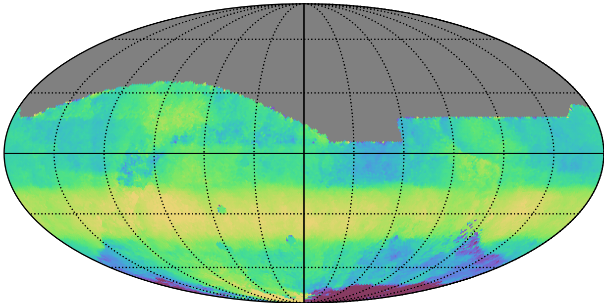
too_elab_r32_d2_gz_v3.4_10yrs All sky r band: Median HA
