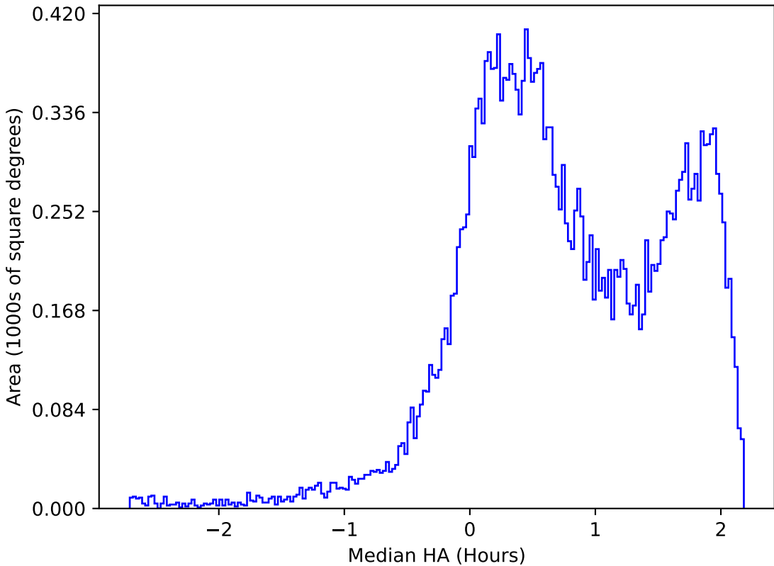
too_elab_r32_d2_gz_v3.4_10yrs All sky r band: Median HA
