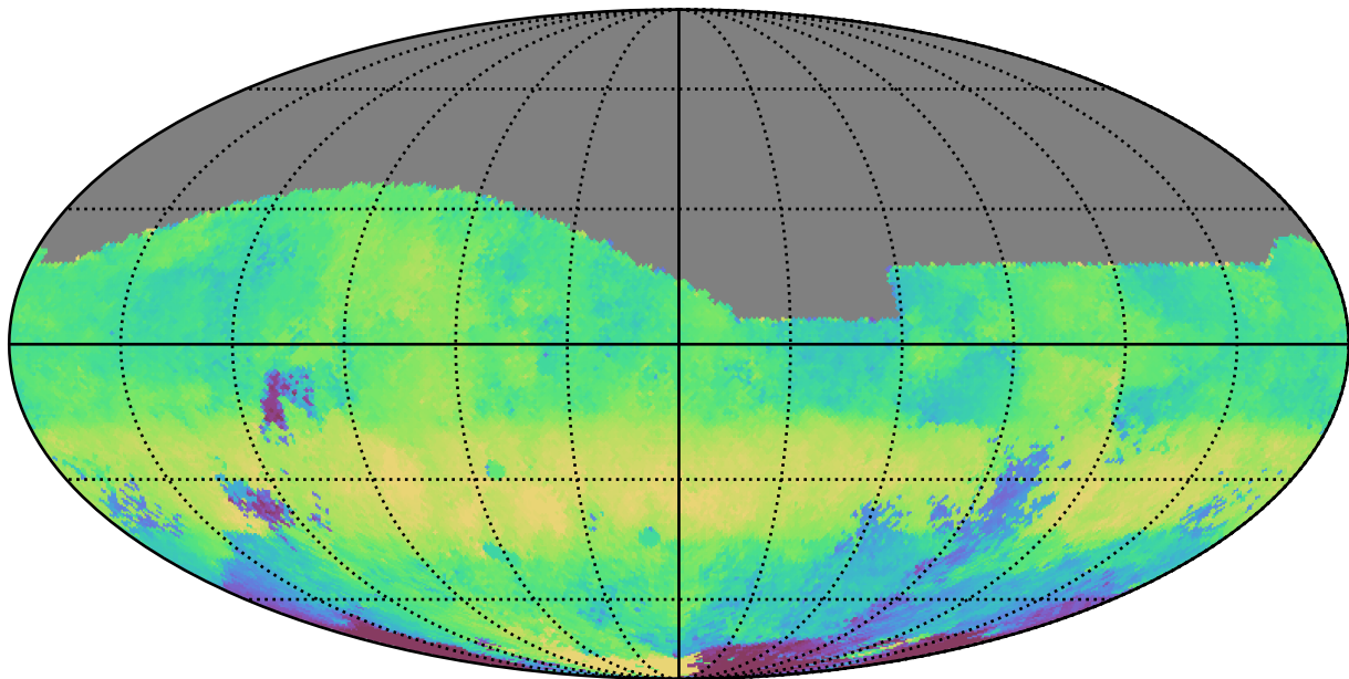
too_elab_r32_d2_gz_v3.4_10yrs All sky g band: Median HA
