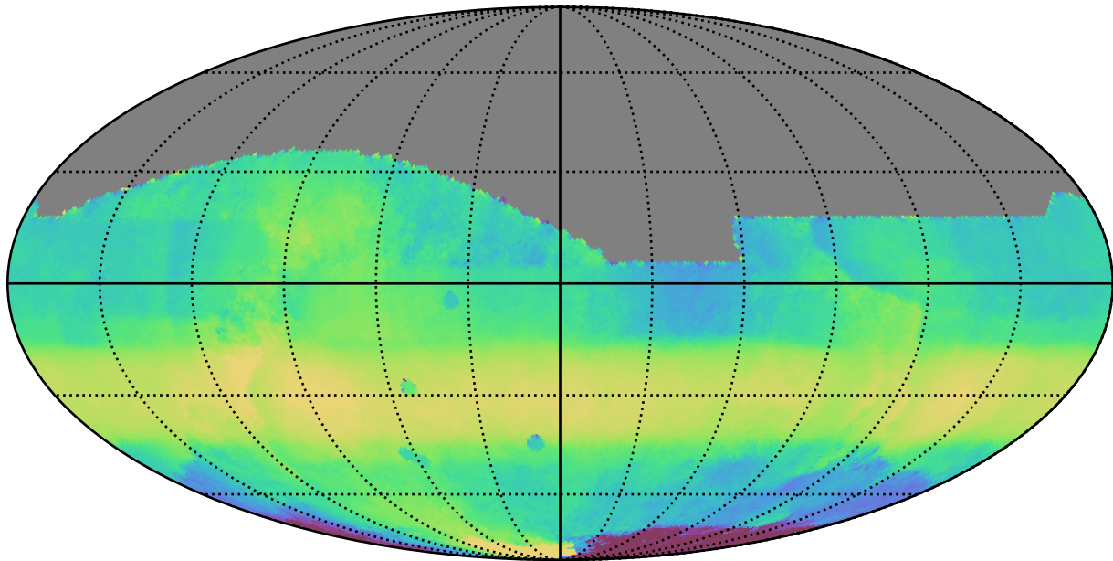
too_elab_r32_d2_gz_v3.4_10yrs All sky all bands: Median HA
