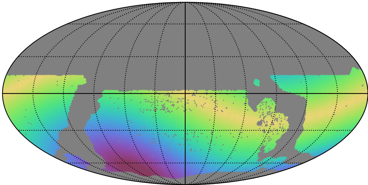
too_elab_r32_d2_gz_v3.4_10yrs WFD y band: Max solarElong
