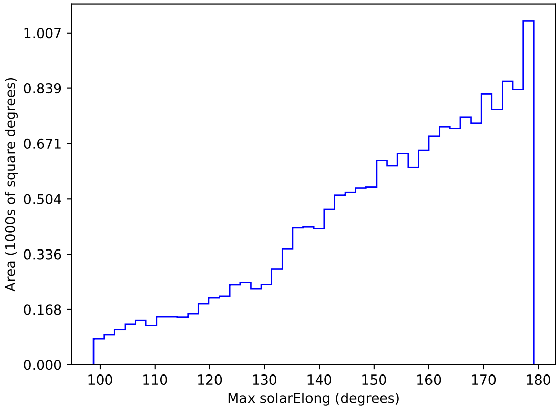
too_elab_r32_d2_gz_v3.4_10yrs WFD y band: Max solarElong
