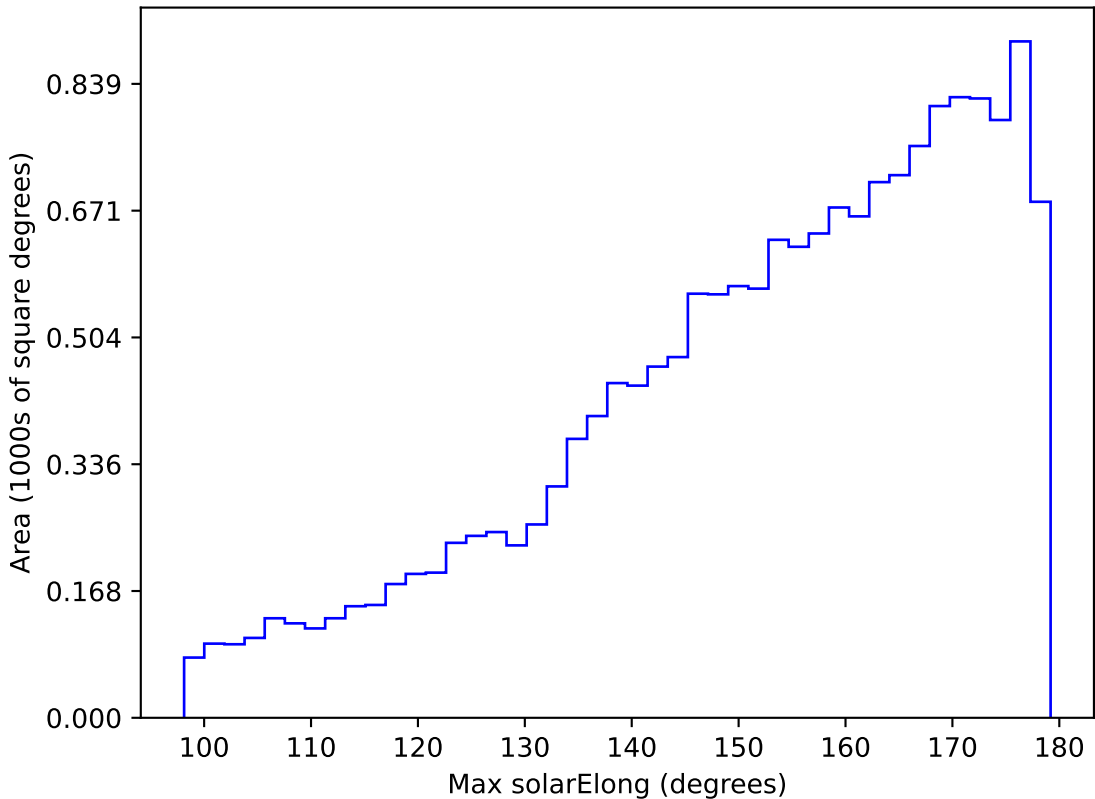
too_elab_r32_d2_gz_v3.4_10yrs WFD u band: Max solarElong
