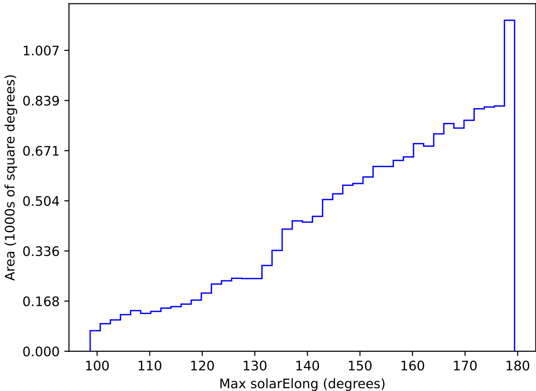
too_elab_r32_d2_gz_v3.4_10yrs WFD r band: Max solarElong
