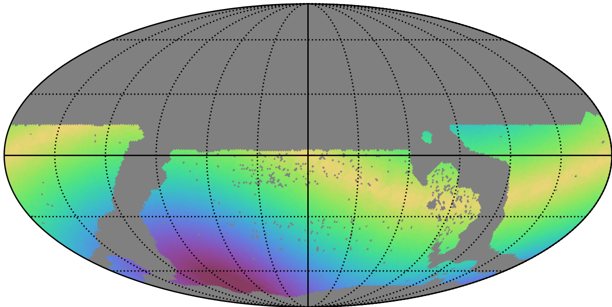
too_elab_r32_d2_gz_v3.4_10yrs WFD g band: Max solarElong
