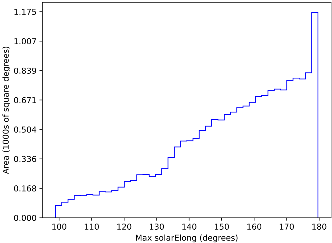
too_elab_r32_d2_gz_v3.4_10yrs WFD all bands: Max solarElong
