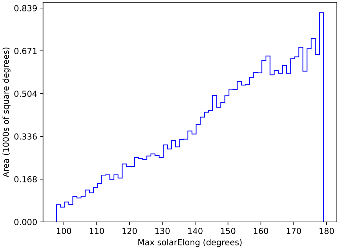
too_elab_r32_d2_gz_v3.4_10yrs All sky y band: Max solarElong
