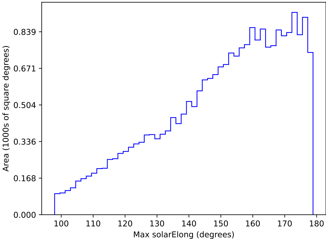
too_elab_r32_d2_gz_v3.4_10yrs All sky u band: Max solarElong
