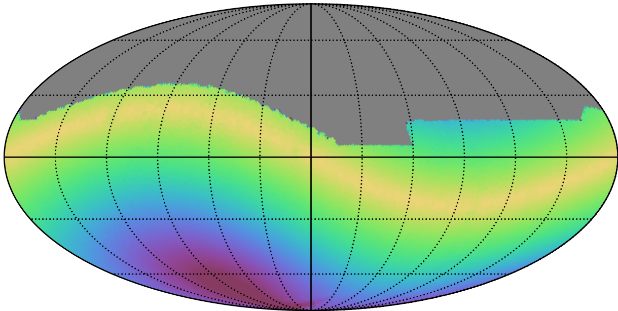
too_elab_r32_d2_gz_v3.4_10yrs All sky r band: Max solarElong
