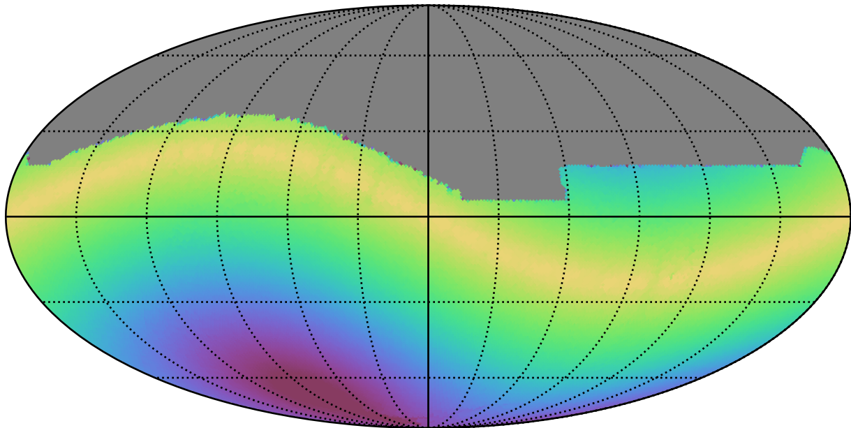
too_elab_r32_d2_gz_v3.4_10yrs All sky i band: Max solarElong
