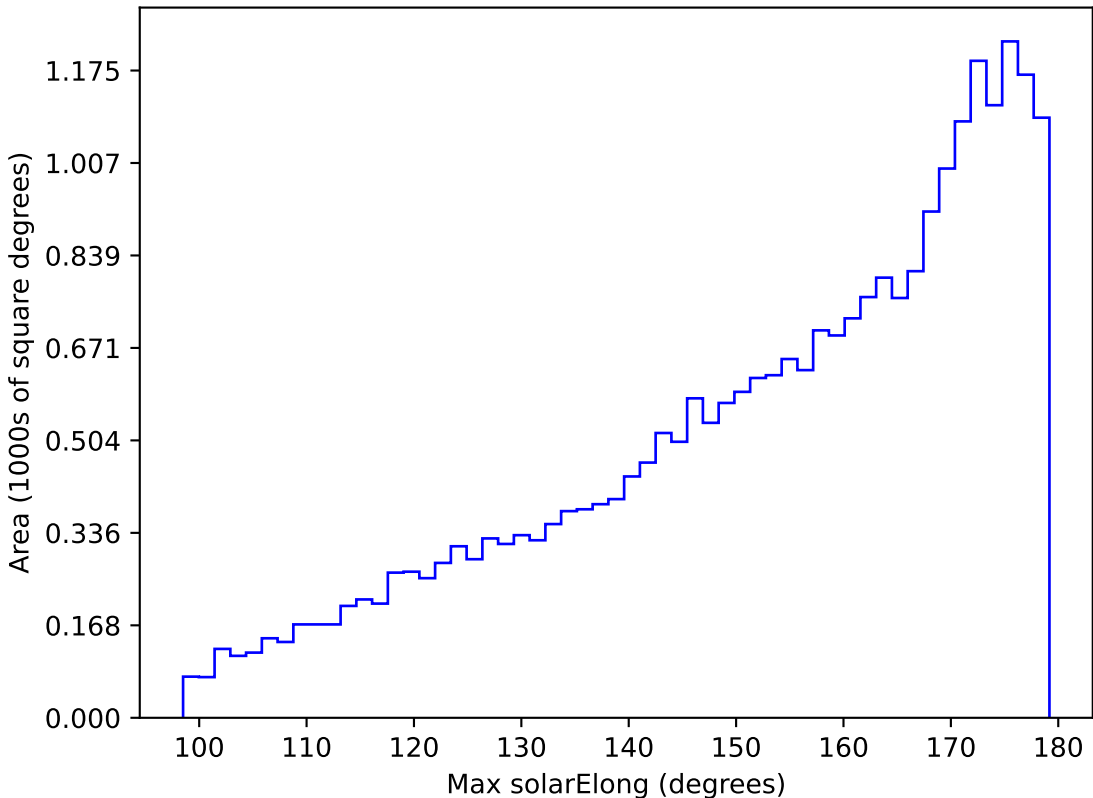
too_elab_r32_d2_gz_v3.4_10yrs All sky g band: Max solarElong
