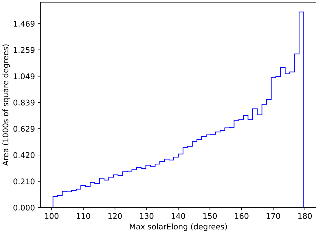
too_elab_r32_d2_gz_v3.4_10yrs All sky all bands: Max solarElong
