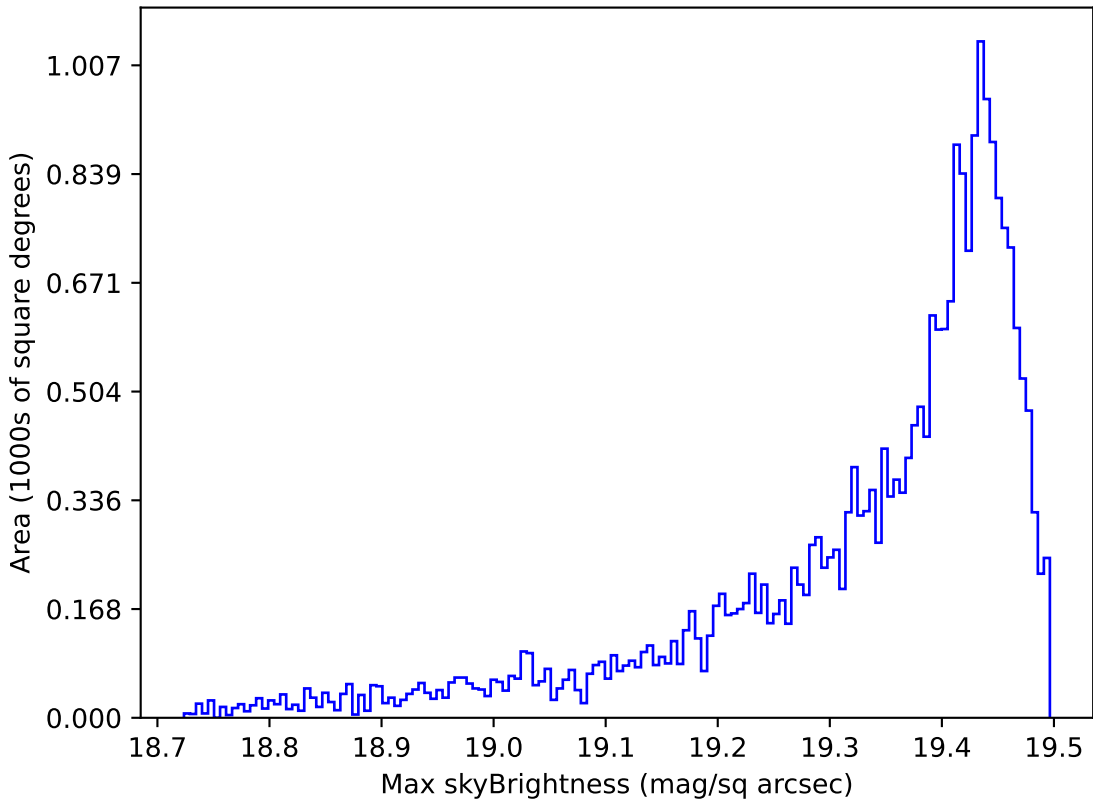
too_elab_r32_d2_gz_v3.4_10yrs Yr 1 z band: Max skyBrightness
