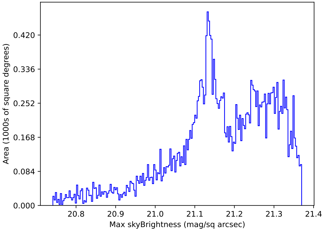
too_elab_r32_d2_gz_v3.4_10yrs Yr 1 r band: Max skyBrightness
