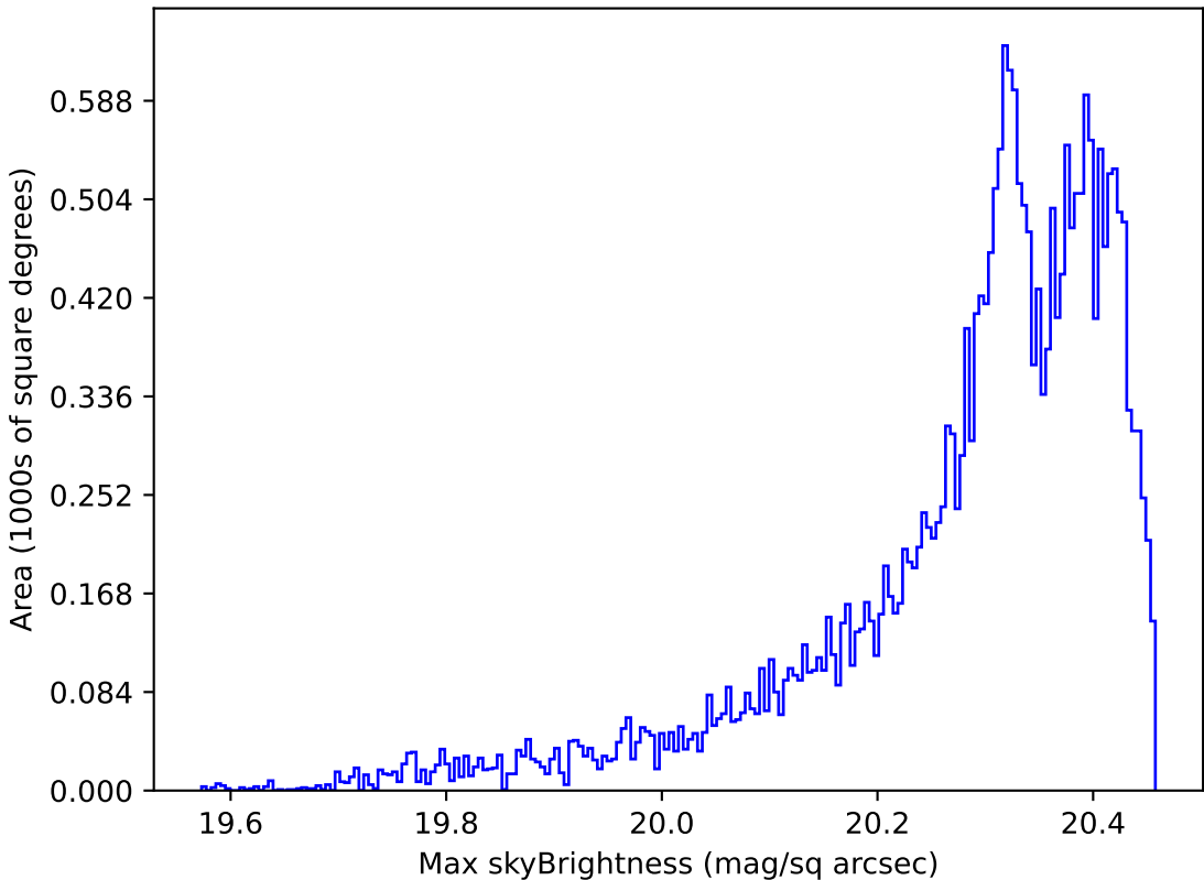
too_elab_r32_d2_gz_v3.4_10yrs Yr 1 i band: Max skyBrightness
