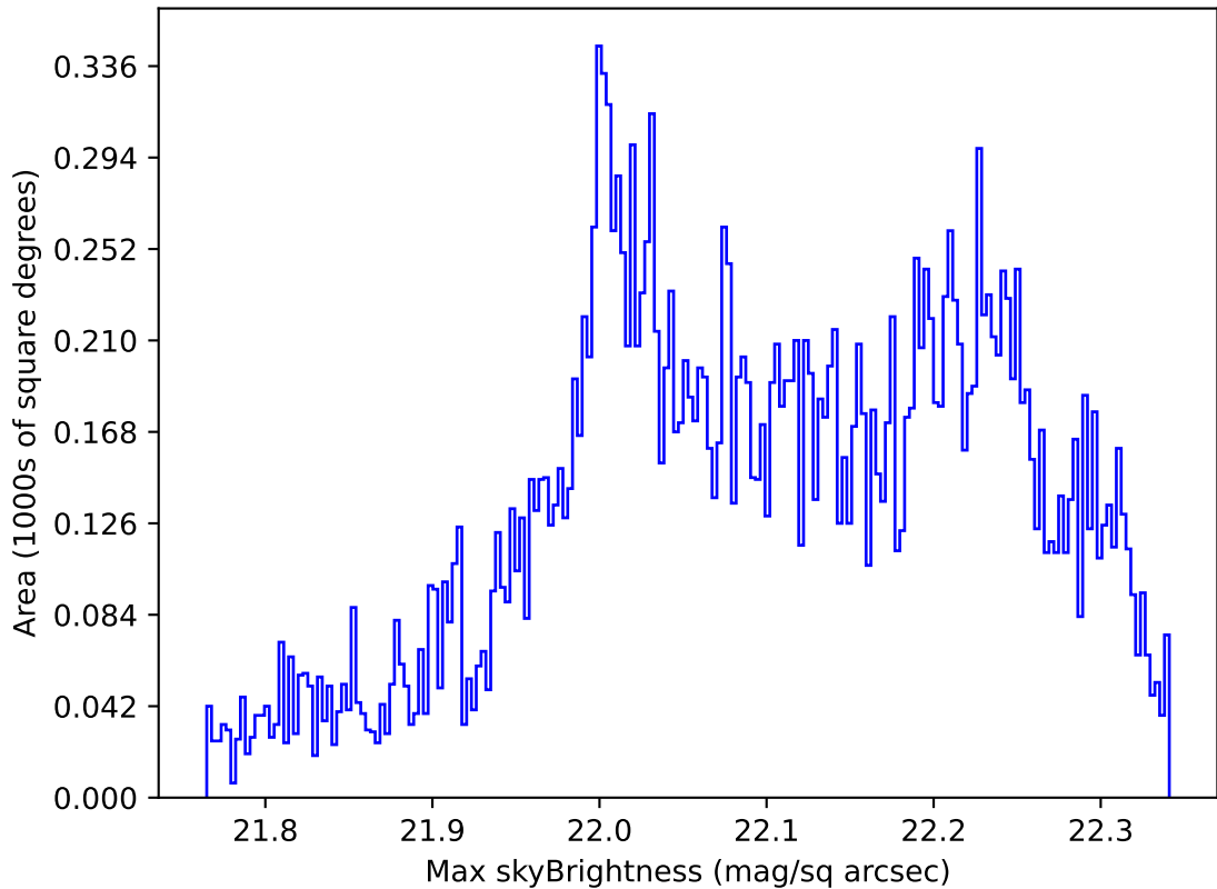
too_elab_r32_d2_gz_v3.4_10yrs Yr 1 g band: Max skyBrightness
