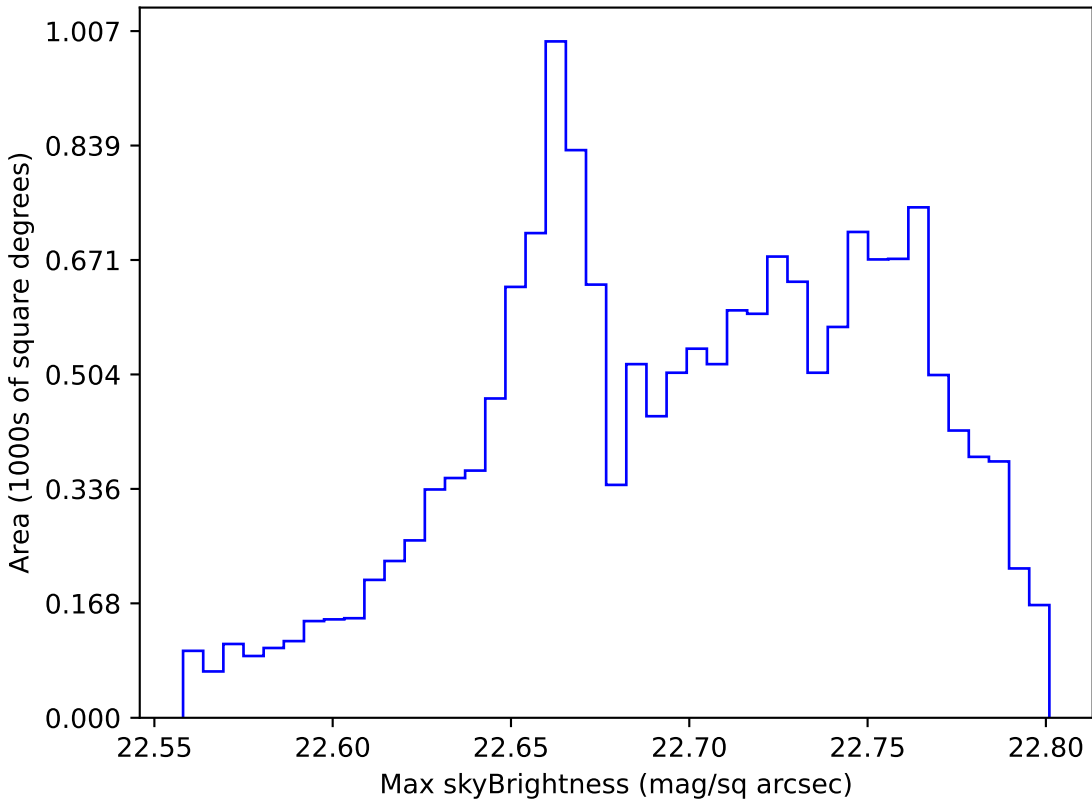
too_elab_r32_d2_gz_v3.4_10yrs WFD u band: Max skyBrightness
