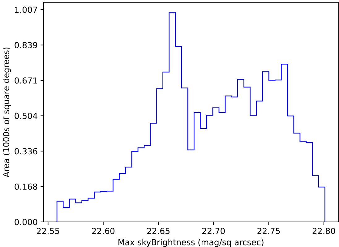
too_elab_r32_d2_gz_v3.4_10yrs WFD all bands: Max skyBrightness
