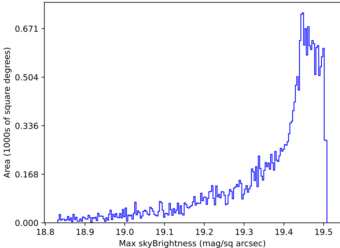
too_elab_r32_d2_gz_v3.4_10yrs All sky z band: Max skyBrightness
