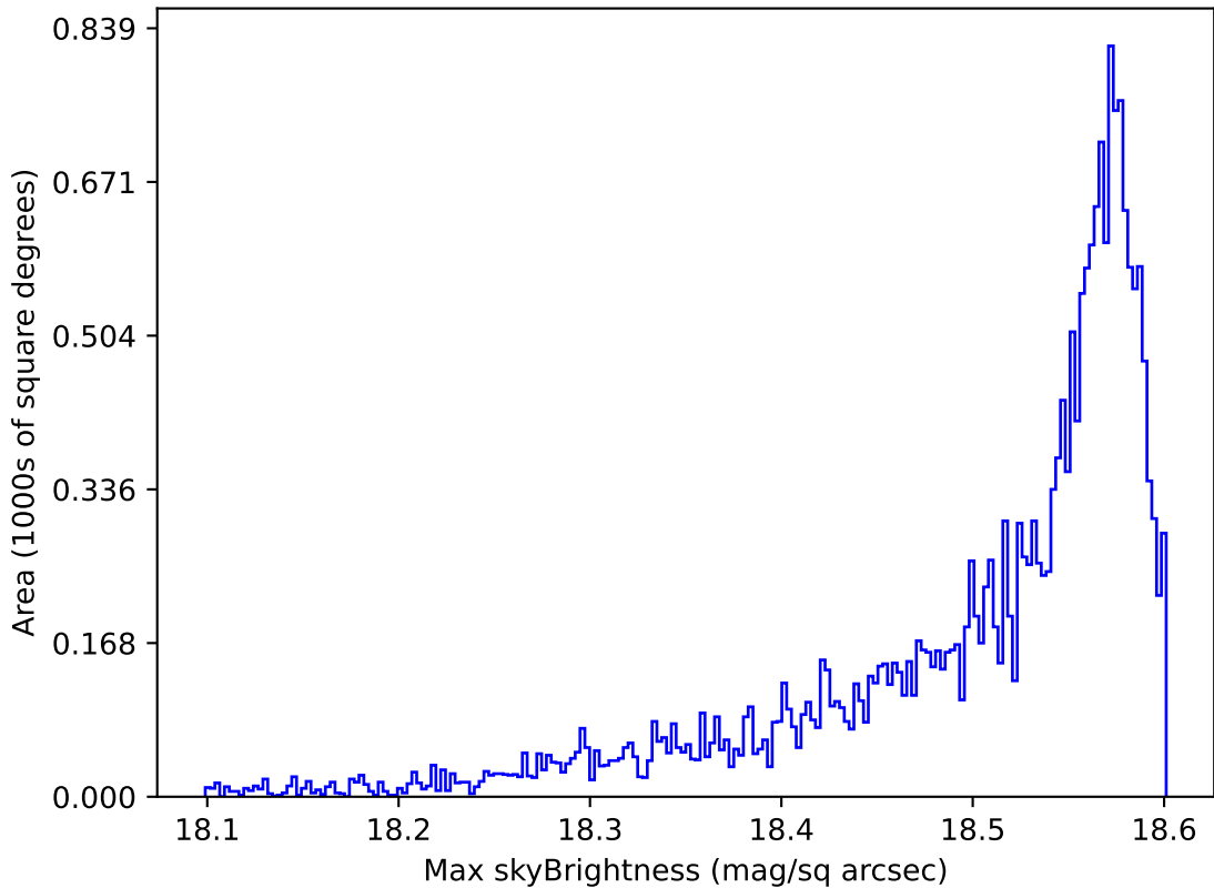
too_elab_r32_d2_gz_v3.4_10yrs All sky y band: Max skyBrightness
