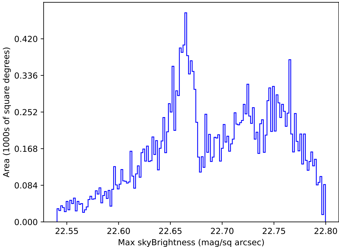
too_elab_r32_d2_gz_v3.4_10yrs All sky u band: Max skyBrightness
