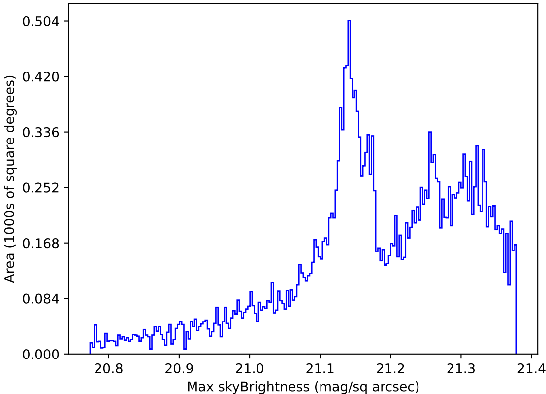
too_elab_r32_d2_gz_v3.4_10yrs All sky r band: Max skyBrightness
