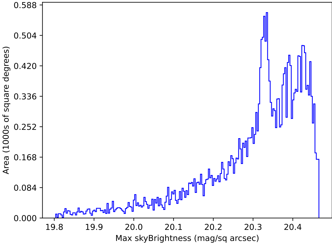
too_elab_r32_d2_gz_v3.4_10yrs All sky i band: Max skyBrightness
