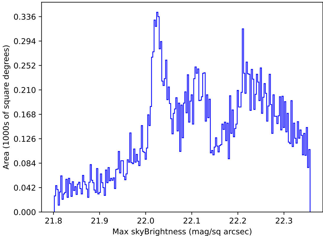
too_elab_r32_d2_gz_v3.4_10yrs All sky g band: Max skyBrightness
