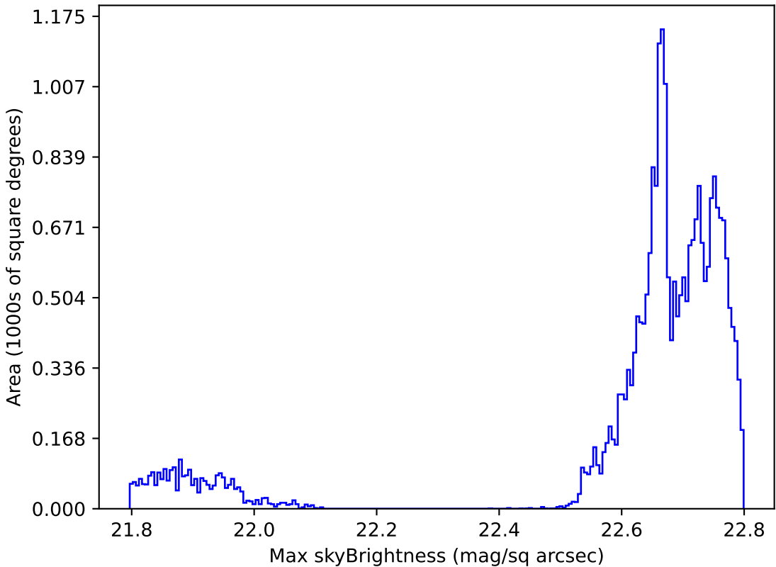
too_elab_r32_d2_gz_v3.4_10yrs All sky all bands: Max skyBrightness
