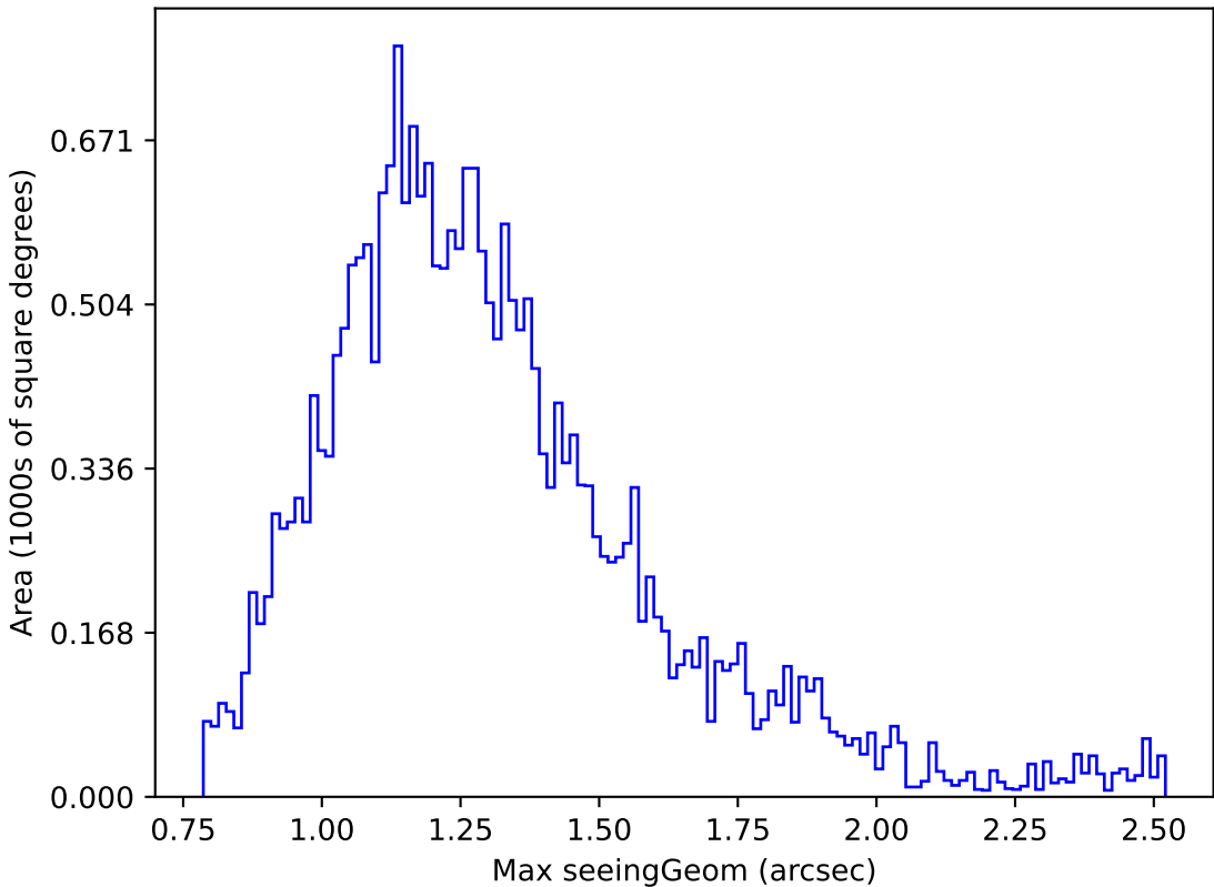
too_elab_r32_d2_gz_v3.4_10yrs Yr 1 z band: Max seeingGeom
