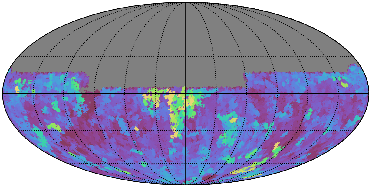
too_elab_r32_d2_gz_v3.4_10yrs Yr 1 y band: Max seeingGeom
