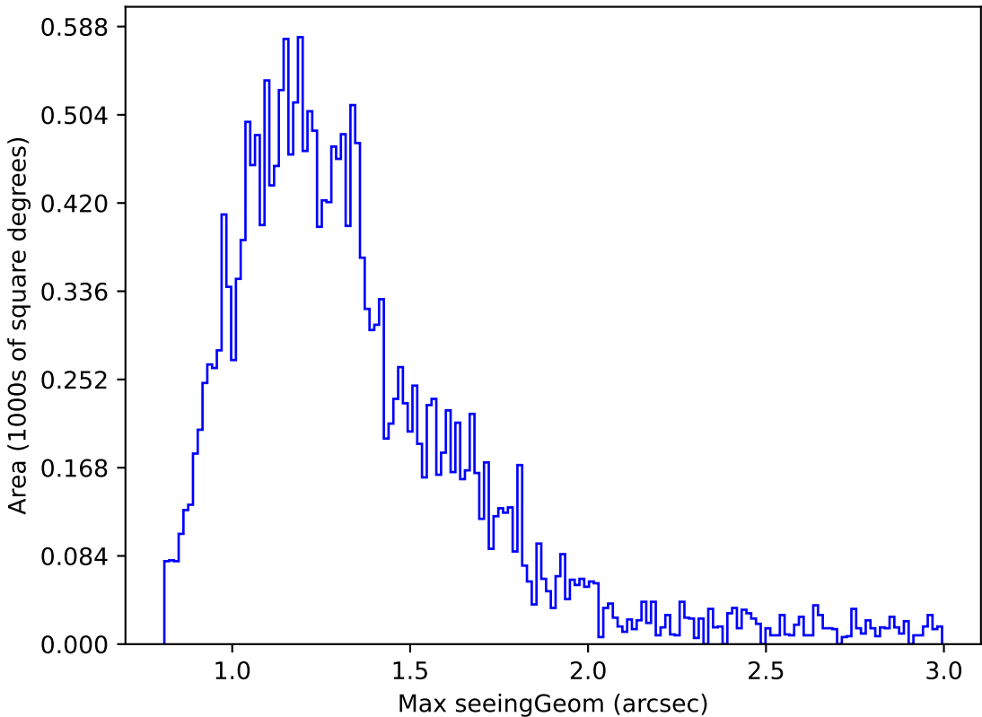
too_elab_r32_d2_gz_v3.4_10yrs Yr 1 u band: Max seeingGeom
