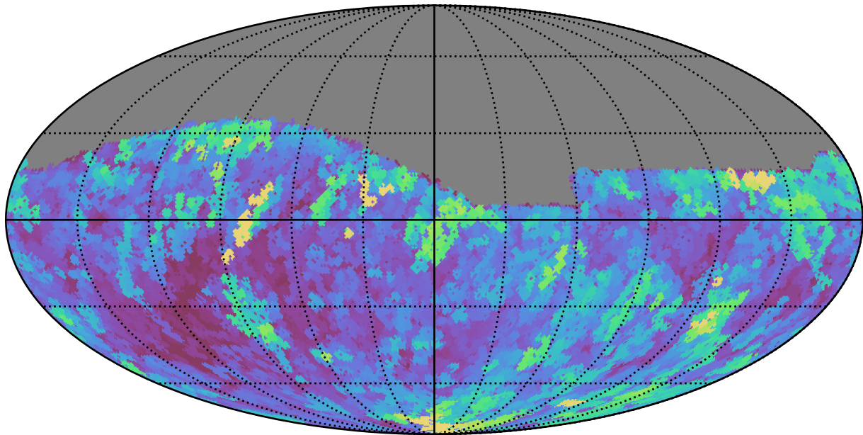
too_elab_r32_d2_gz_v3.4_10yrs Yr 1 r band: Max seeingGeom
