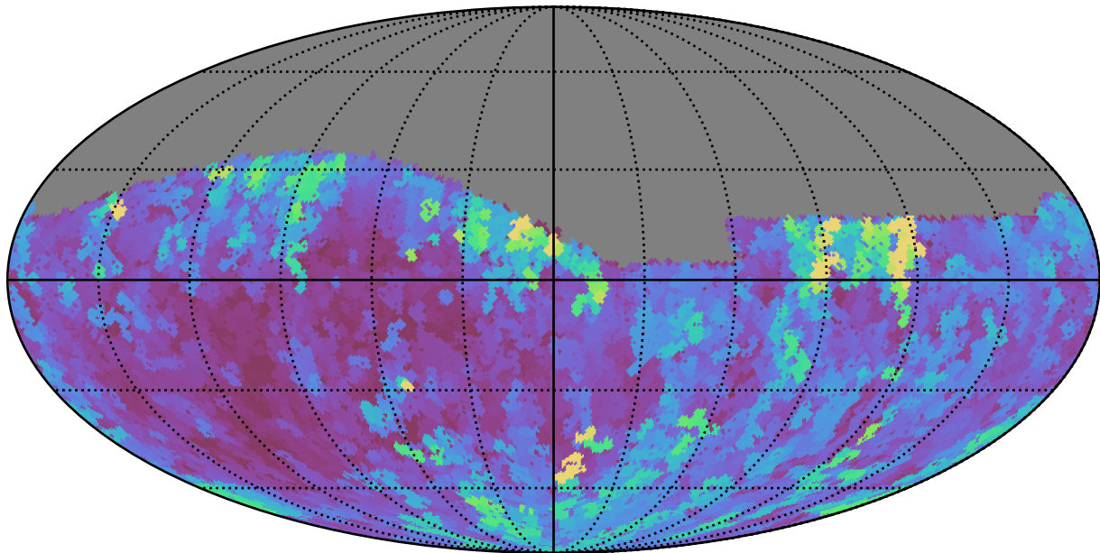
too_elab_r32_d2_gz_v3.4_10yrs Yr 1 g band: Max seeingGeom
