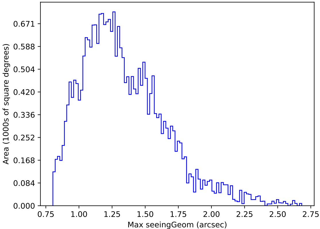
too_elab_r32_d2_gz_v3.4_10yrs Yr 1 g band: Max seeingGeom
