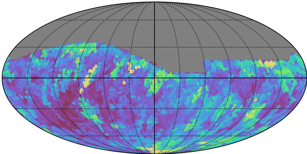
too_elab_r32_d2_gz_v3.4_10yrs Yr 1 r band: Max seeingEff
