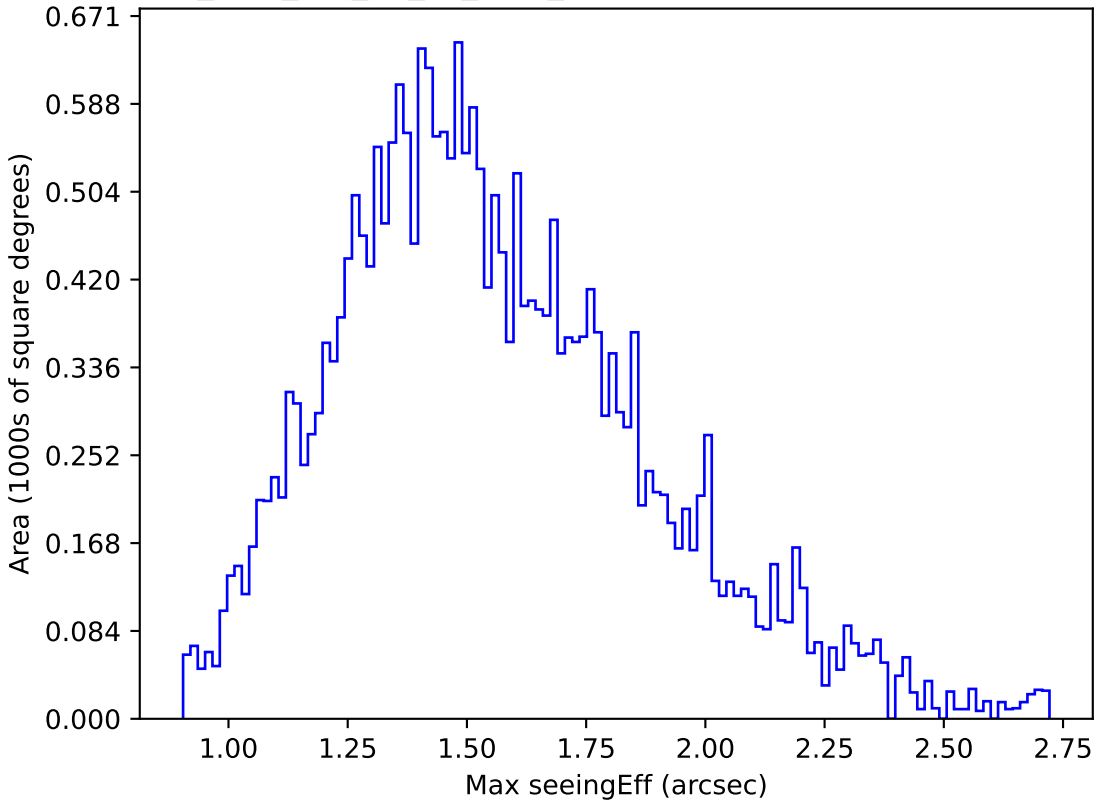
too_elab_r32_d2_gz_v3.4_10yrs Yr 1 r band: Max seeingEff
