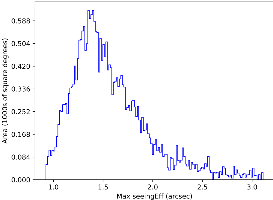
too_elab_r32_d2_gz_v3.4_10yrs Yr 1 i band: Max seeingEff
