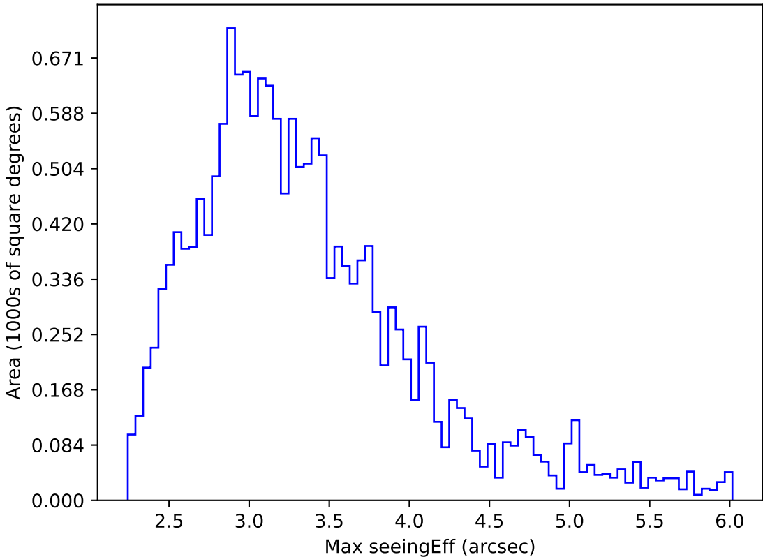
too_elab_r32_d2_gz_v3.4_10yrs WFD all bands: Max seeingEff
