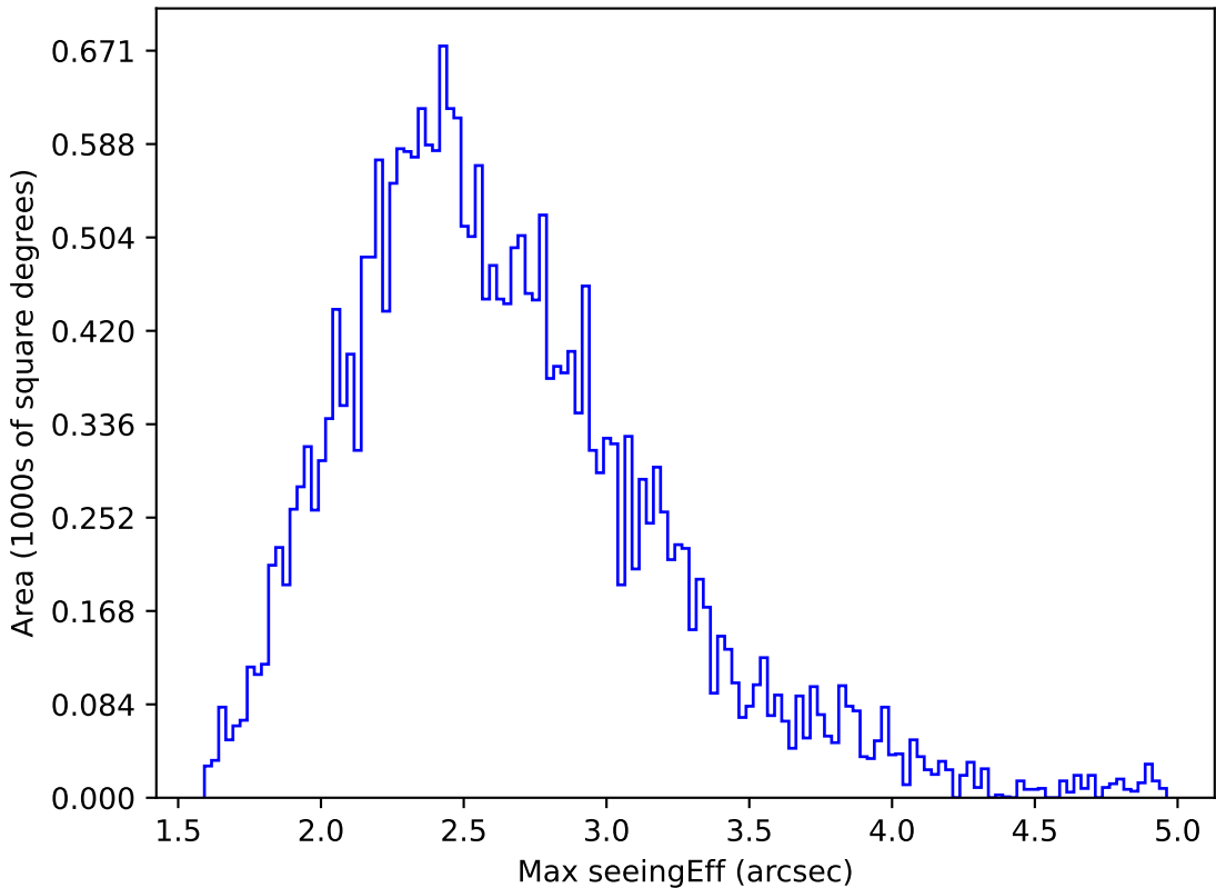
too_elab_r32_d2_gz_v3.4_10yrs All sky r band: Max seeingEff
