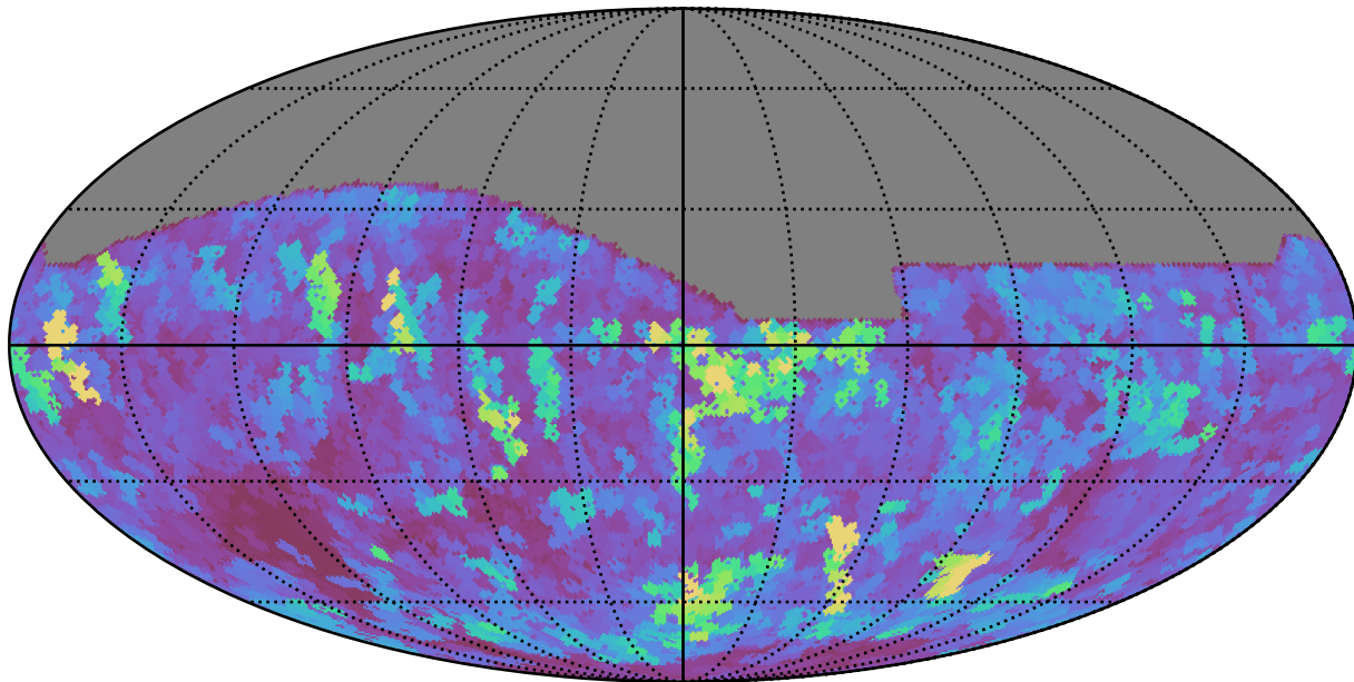
too_elab_r32_d2_gz_v3.4_10yrs All sky i band: Max seeingEff
