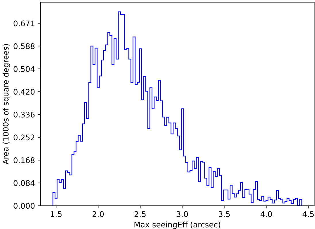
too_elab_r32_d2_gz_v3.4_10yrs All sky g band: Max seeingEff
