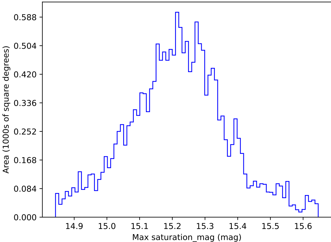
too_elab_r32_d2_gz_v3.4_10yrs WFD z band: Max saturation_mag
