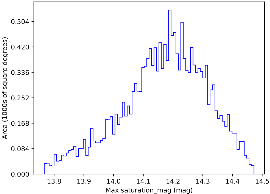
too_elab_r32_d2_gz_v3.4_10yrs WFD y band: Max saturation_mag
