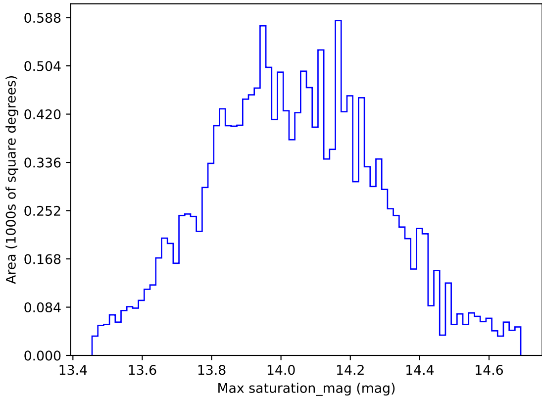
too_elab_r32_d2_gz_v3.4_10yrs WFD u band: Max saturation_mag
